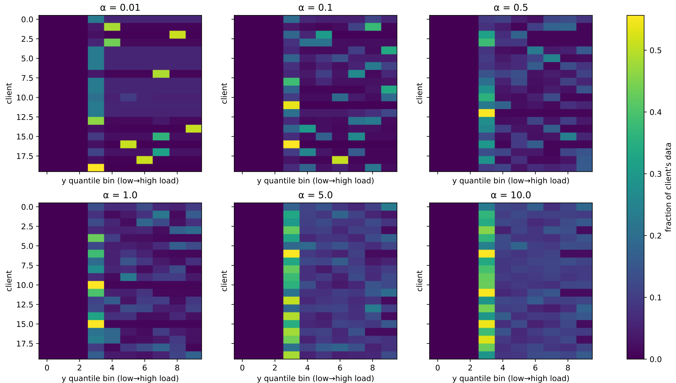
Per-client label (y-bin) distribution — low \alpha should look striped, high \alpha uniform
